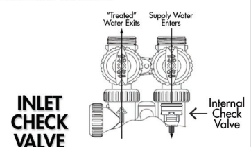
Note Internal Check Valve on the Inlet of the Control
